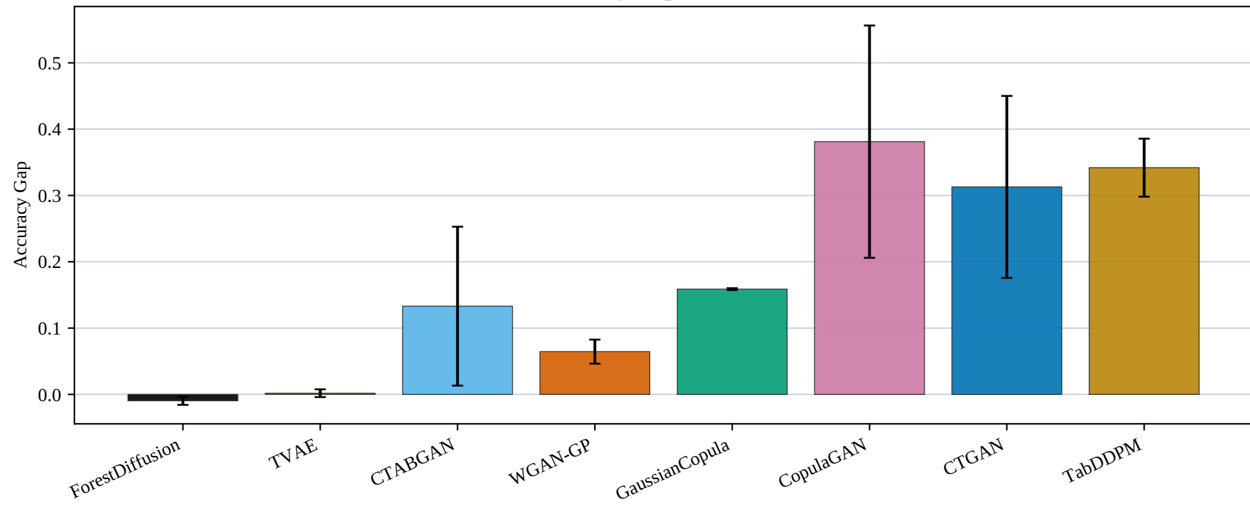
Cancer — Accuracy Gap (mean \pm SD, 10 seeds)
